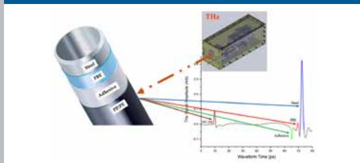
Fig.1 Simplified 3LC Pipe illustration “ToF” principle:
