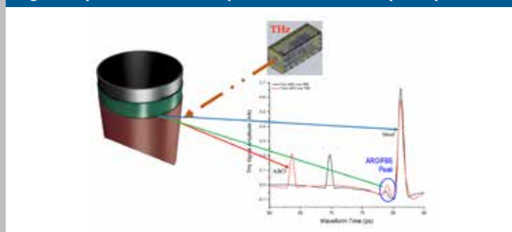
Fig.2 Simplified FBE/ARO Pipe illustration “ToF” principle:
